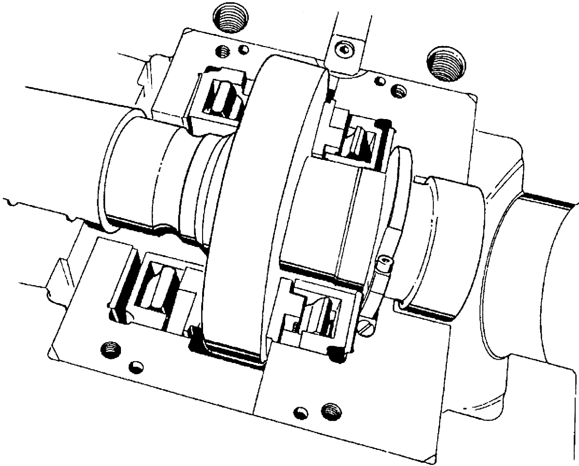
Figure 231-2-10 Thrust Bearing Collar
