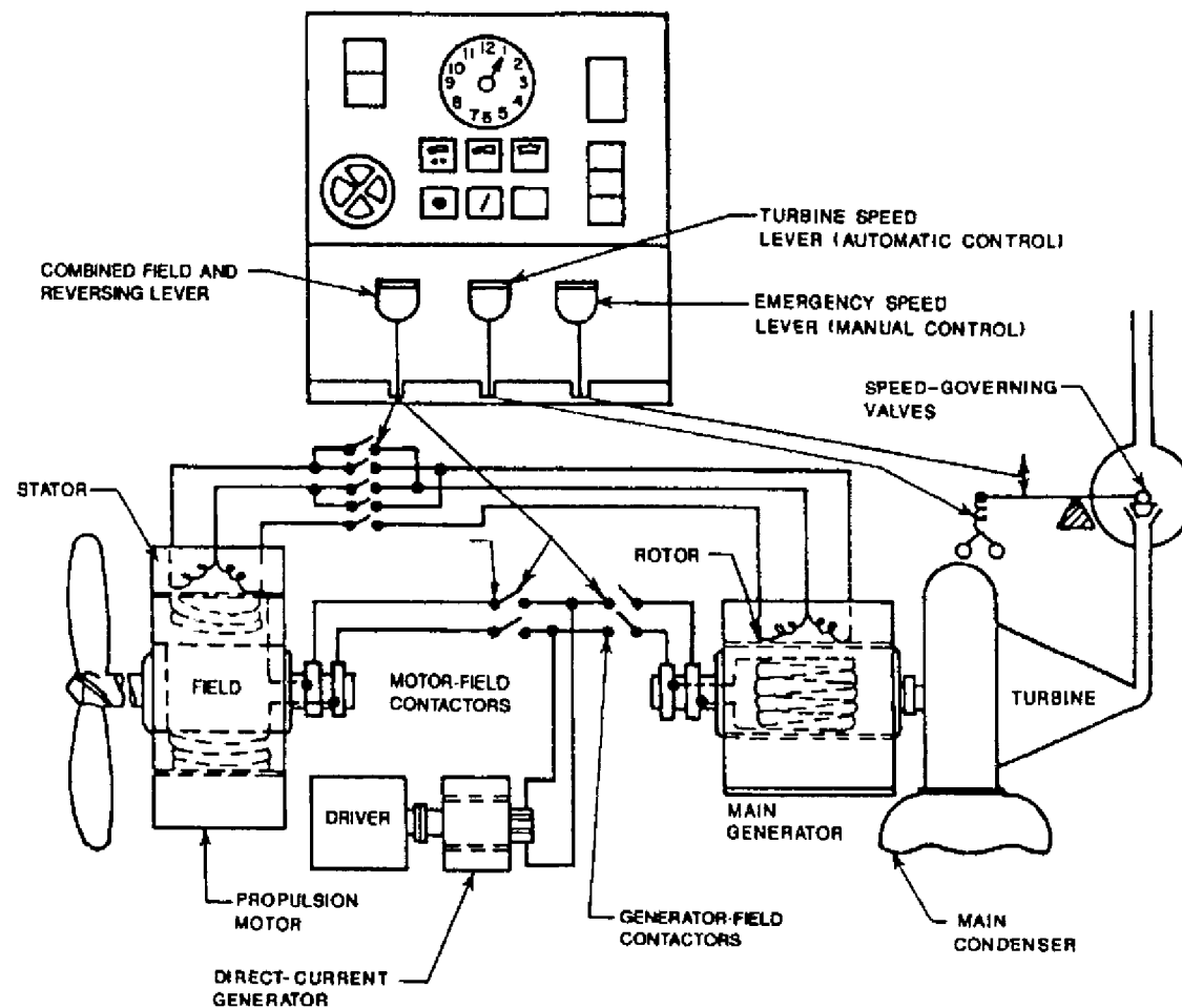
Figure 231-2-3 Diagram of the Turboelectric Drive for Surface Ships
