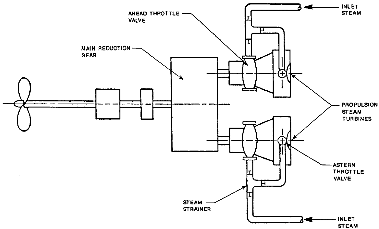
Figure 231-2-1 Typical Main Propulsion Steam Turbine Arrangement for Submarines
