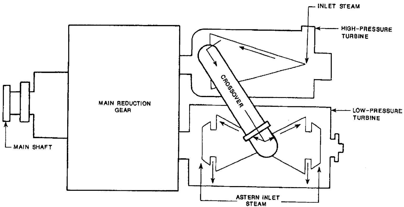
Figure 231-2-2 Geared Cross-Compound Main Propulsion Steam Turbine
