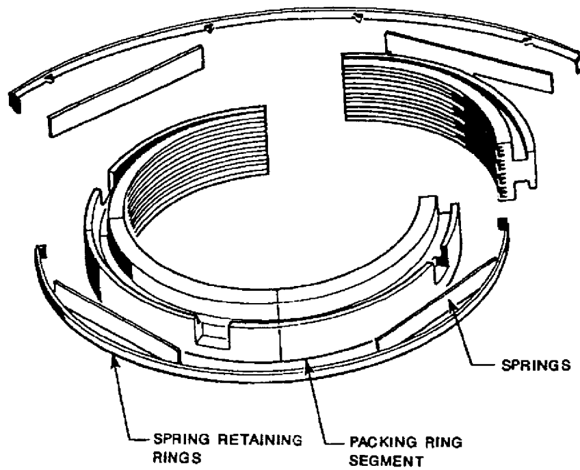
Figure 231-2-7 Shaft Packing
