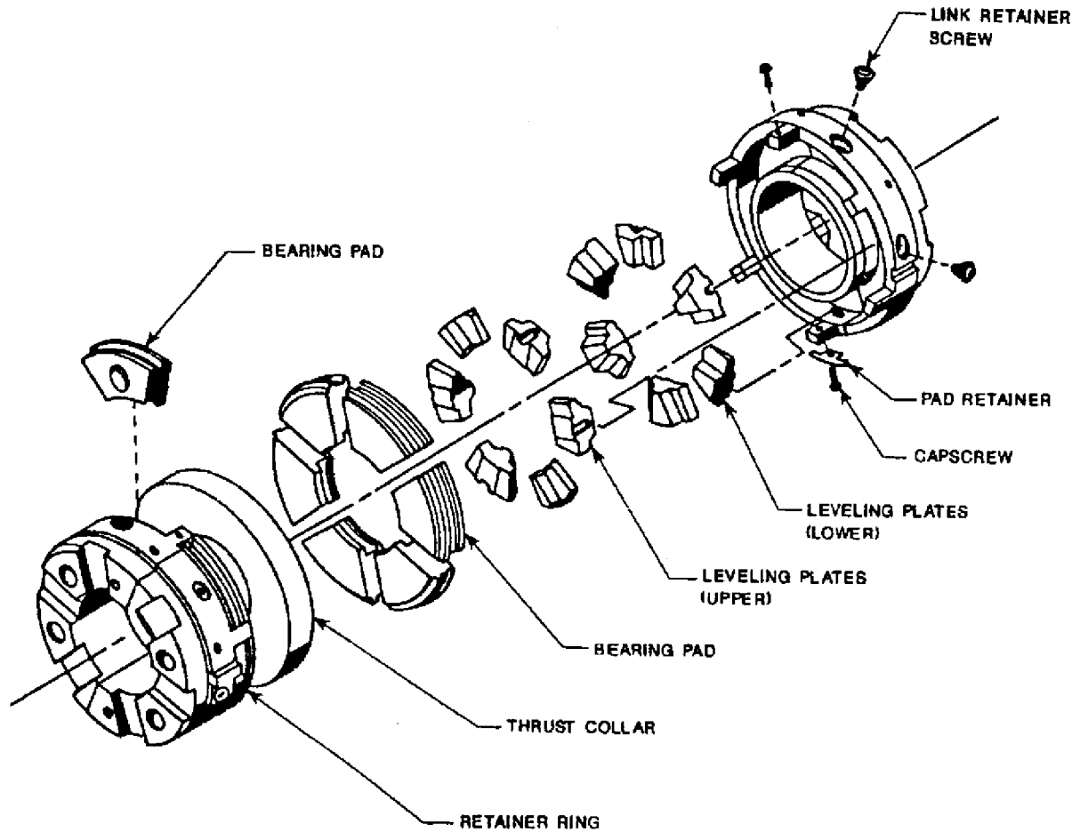
Figure 231-2-9 Thrust Bearing (Exploded View)
