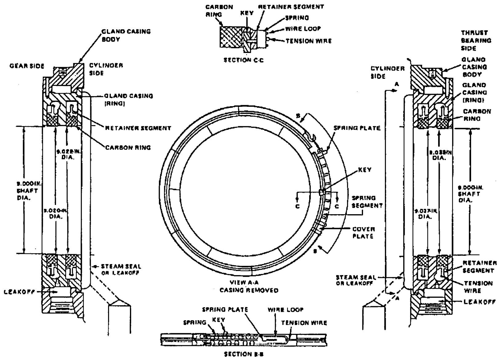
Figure 231-2-6 Shaft Packing Gland Rings (Carbon)
