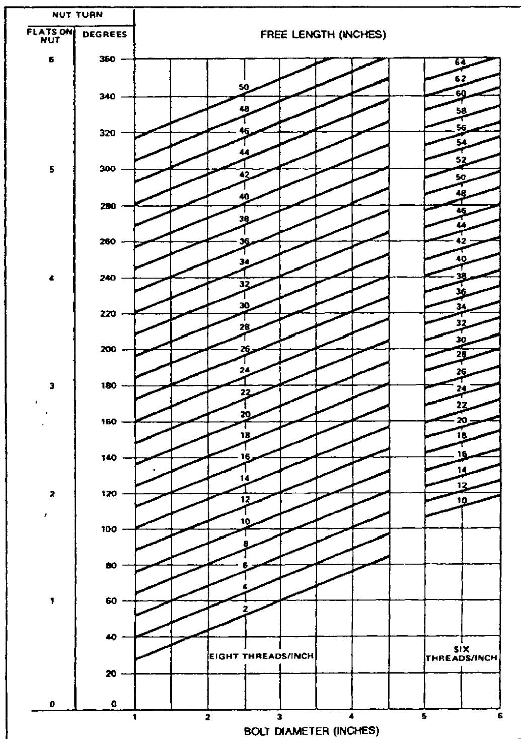
Figure 231-8-9 Alloy-Steel Bolting Nut-Turn Chart
