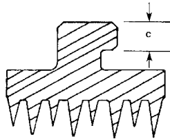
Figure 231-8-4 Packing Ring
