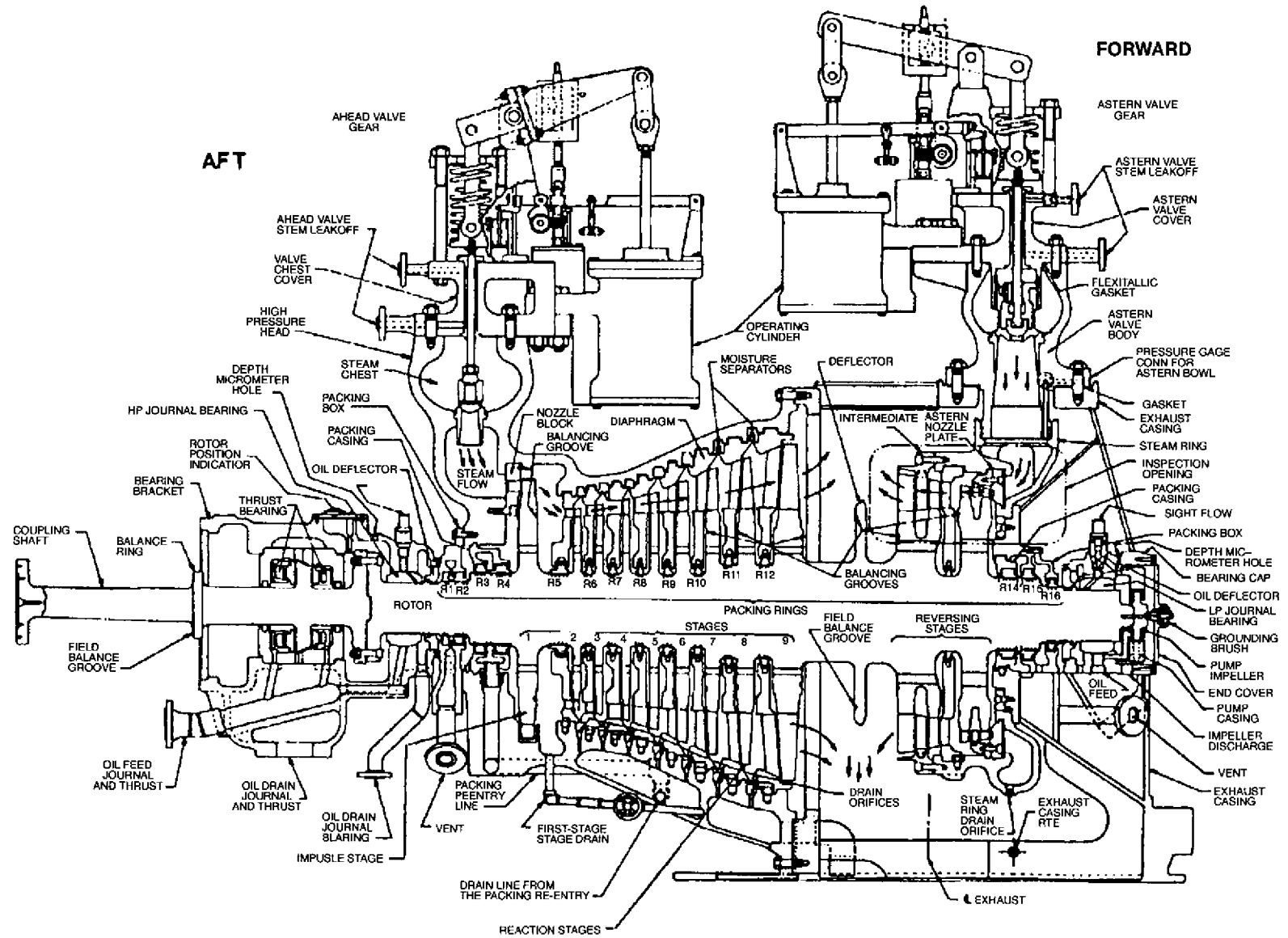
Figure 231-2-4 Single-Casing Propulsion Steam Turbine Longitudinal Section
