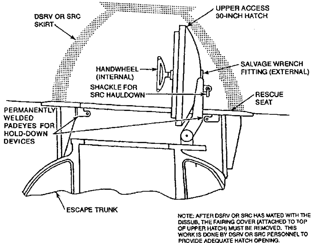
Figure 594-2-2 Features of Typical Rescue/Escape Trunk with 30-Inch Upper Access Hatch
