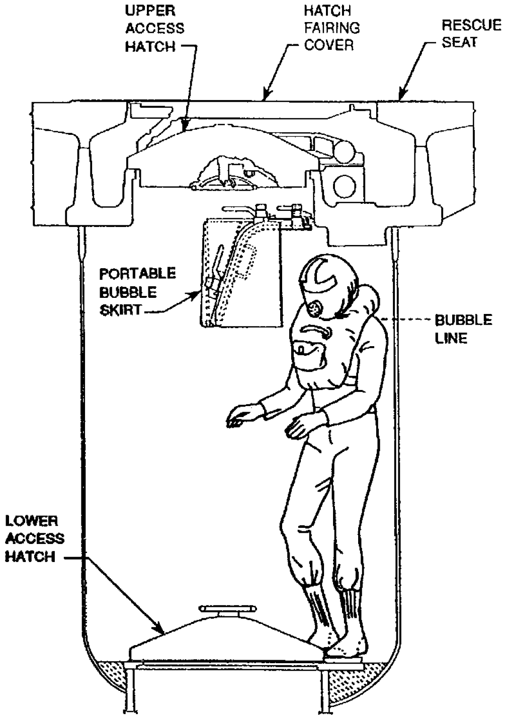
Figure 594-4-5 Typical Rescue/Escape Trunk with Portable Skirt on SSN 688 and Later Classes
