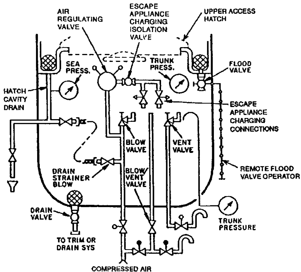
Figure 594-4-6 Typical Rescue/Escape Trunk Features
