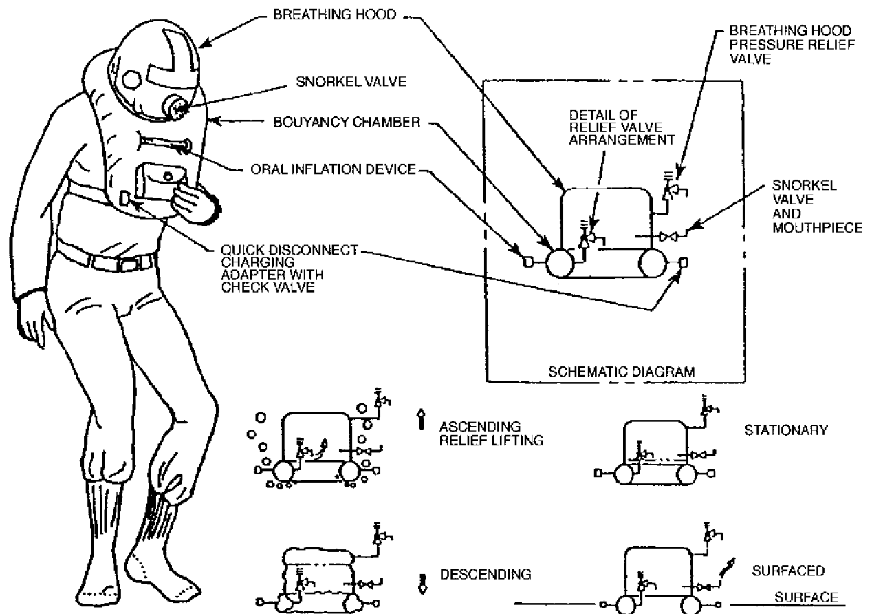
Figure 594-4-1 Submarine Escape Appliance
