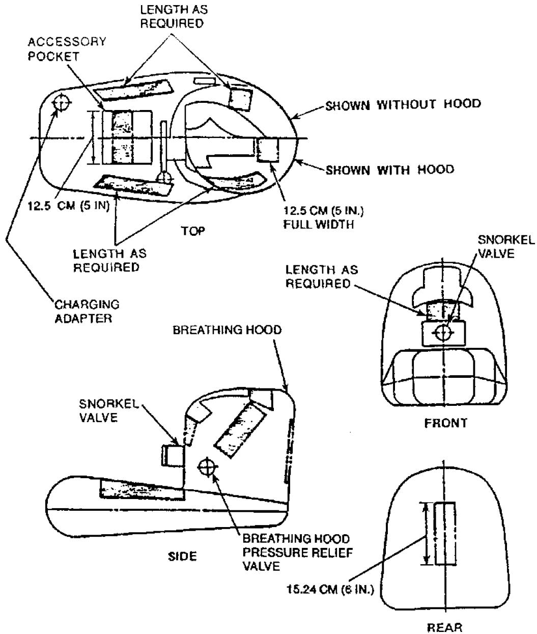
Figure 594-4-3 Reflective Tape Applied to Submarine Escape Appliance
