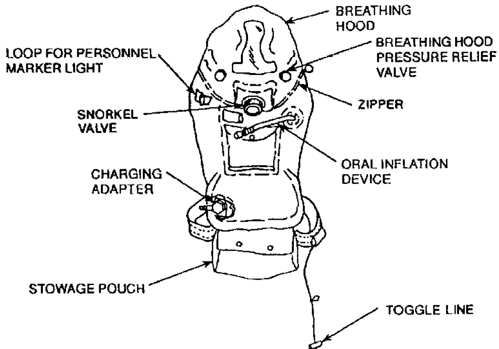
Figure 594-4-2 Detail View of Submarine Escape Appliance Features (Reflective Tape Not Shown)
