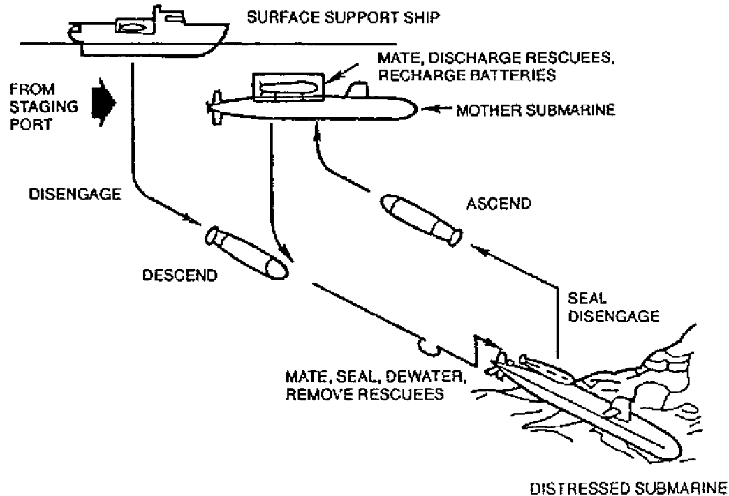
Figure 594-3-2 Typical Sequence of Events During DSRV Rescue Operation
