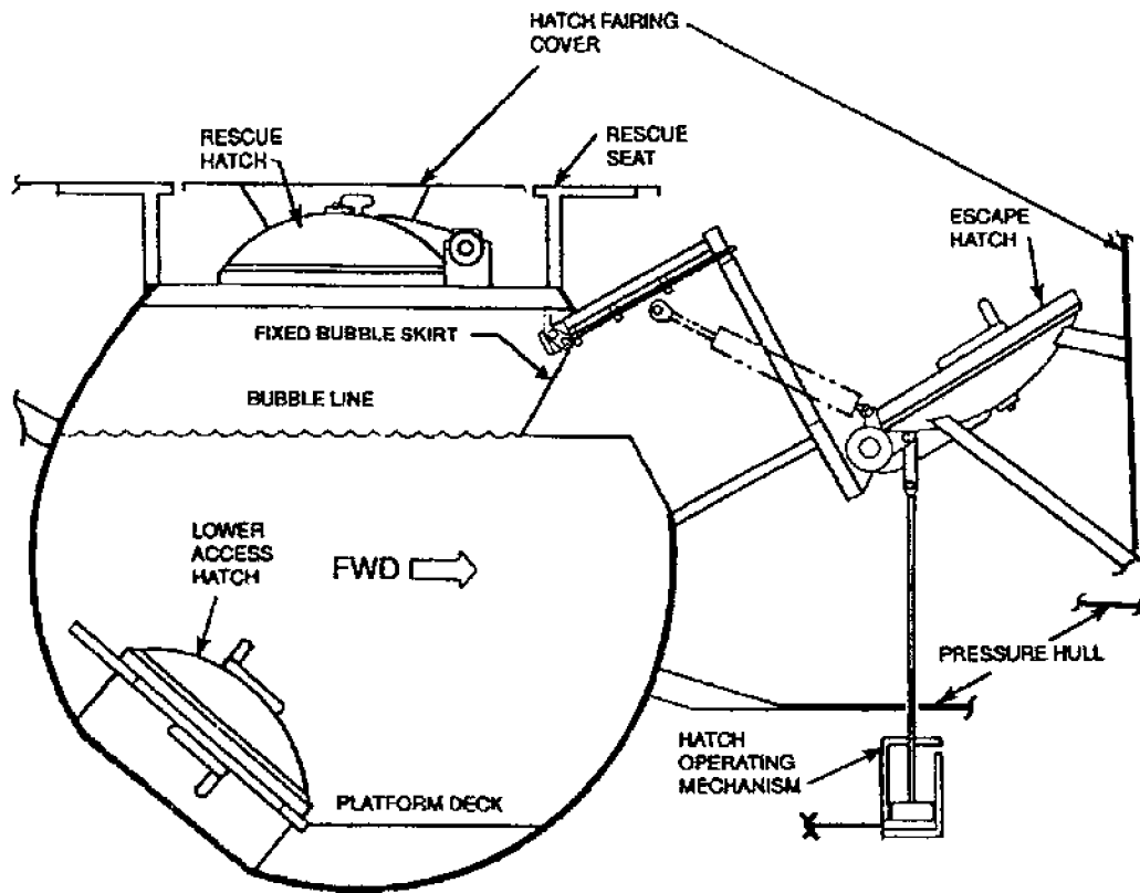
Figure 594-4-4 Typical Rescue/Escape Trunk on SSN 637 and Earlier Classes
