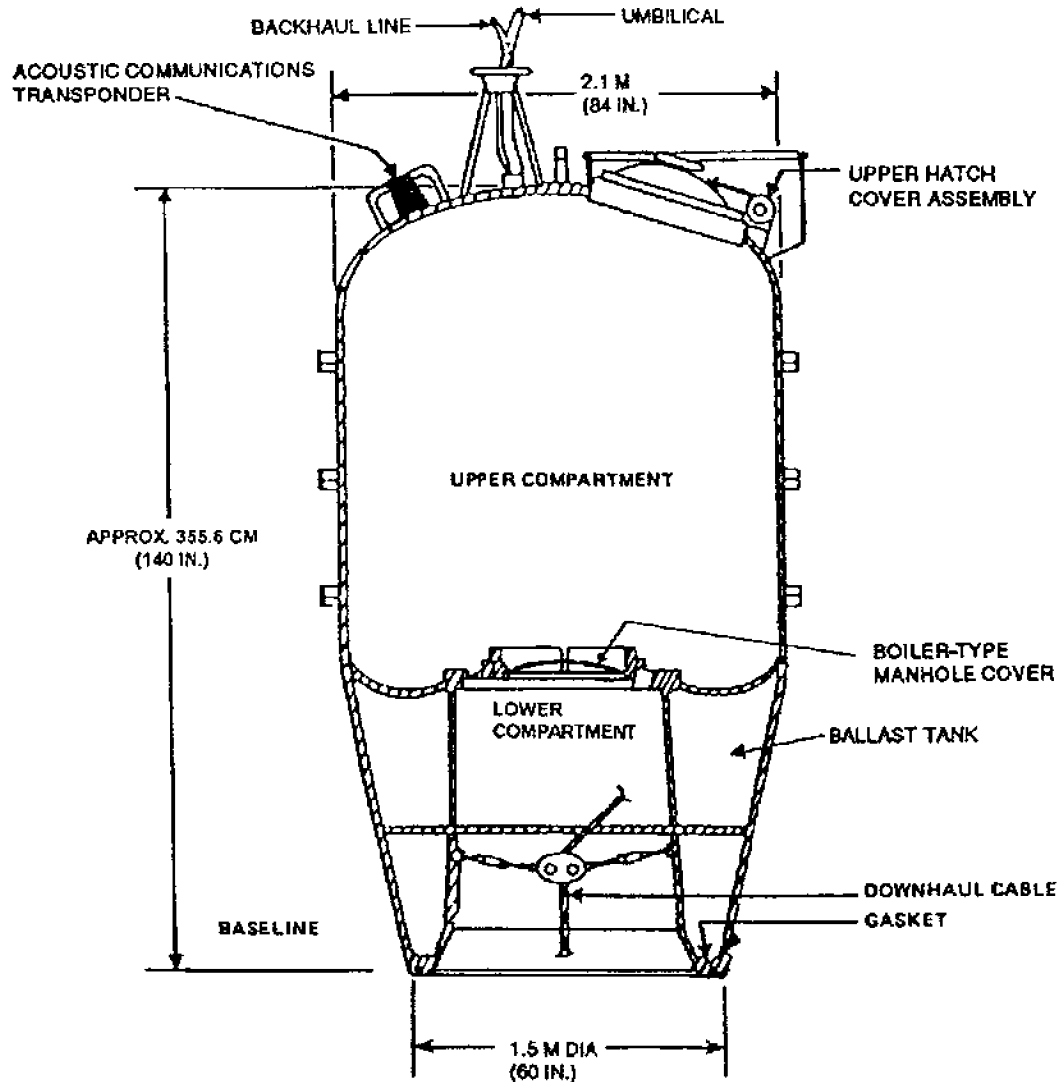
Figure 594-2-1 Submarine Rescue Chamber
